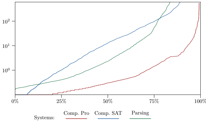
Figure 1: Solved “valid” instances relative to runtime in seconds (TO setting, with method preconditions).
